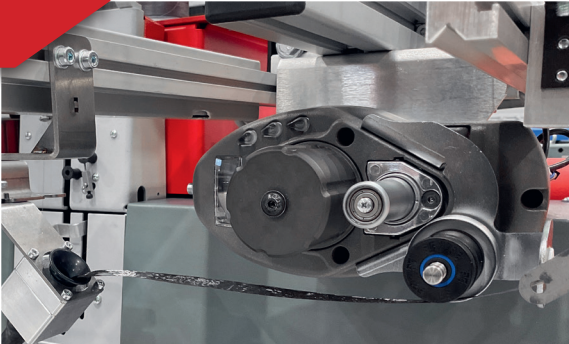
Digital Tensioning
