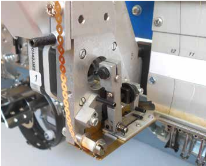
SEQUIN DEVICE V6.1 Stitch one kind of sequins with size: 3mm up to 9mm
